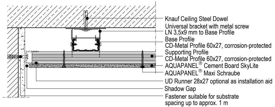
Connection to wall, option 1
