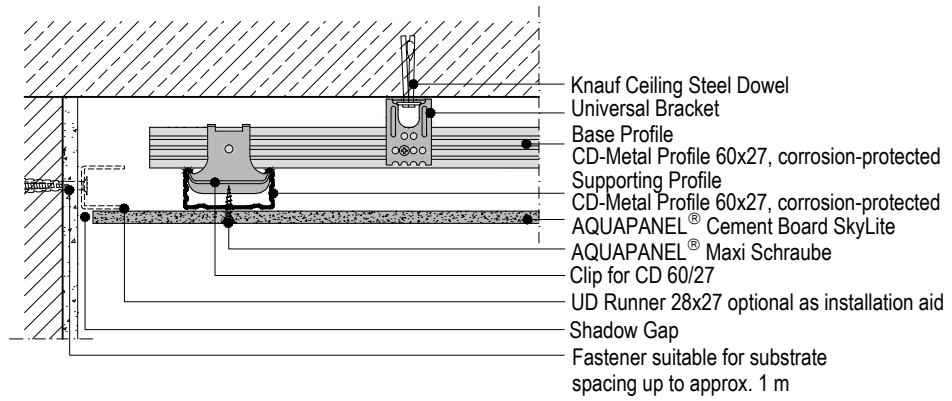
Connection to wall, option 2
