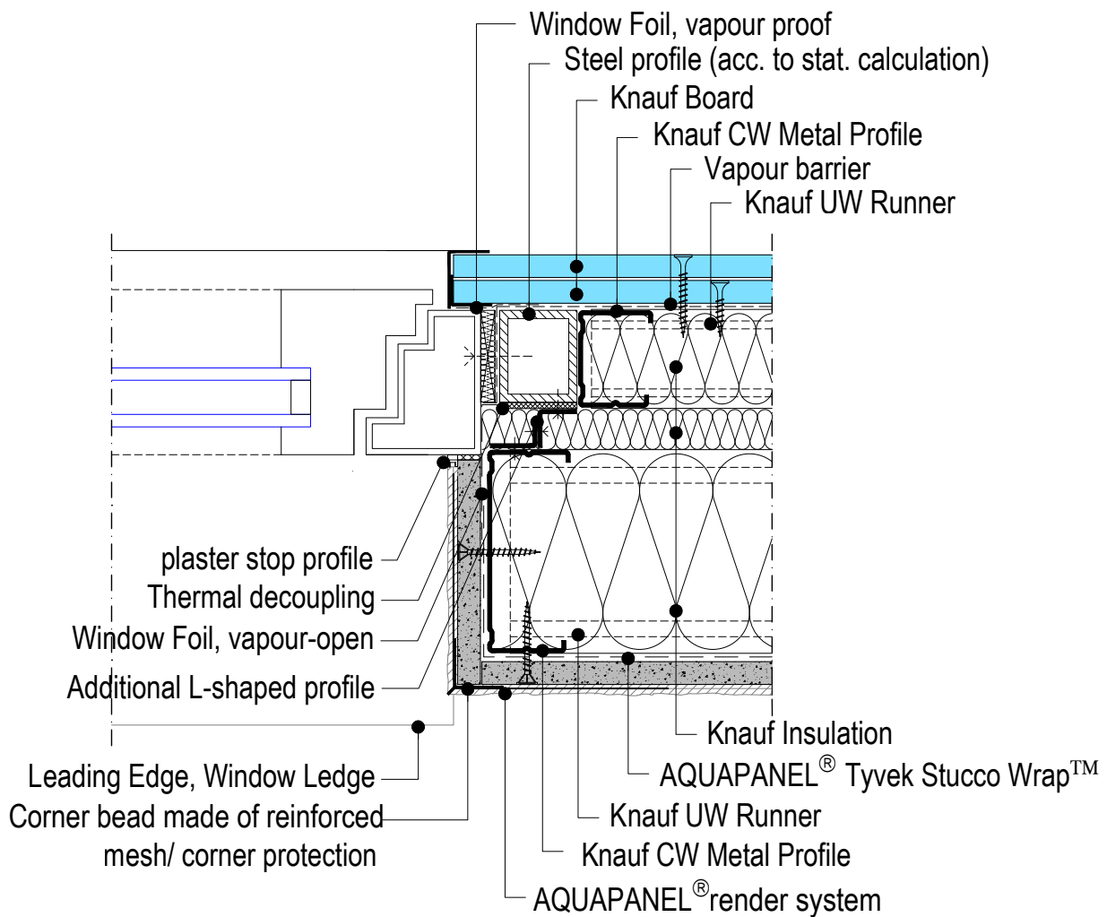
W388E-FE-VM1.en Side connection to window, option 1
